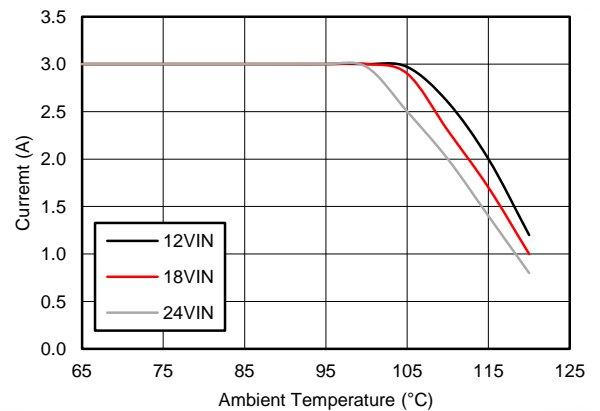
V_{OUT} = 1\text{ V} F_S = 500\text{ kHz} \theta_{JA} = 20^{\circ}\text{C}/\text{W}
