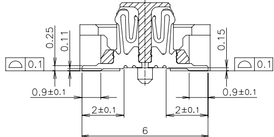
SECT. Y-Y (SIGNAL POSITION) (SCALE 8:1)
