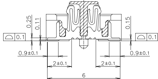
SECT. Z-Z (GROUND POSITION) (SCALE 8:1)
