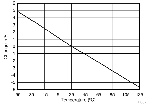
Figure 9. Sampling Period Change vs Temperature (1.7 V to 5.5 V)
