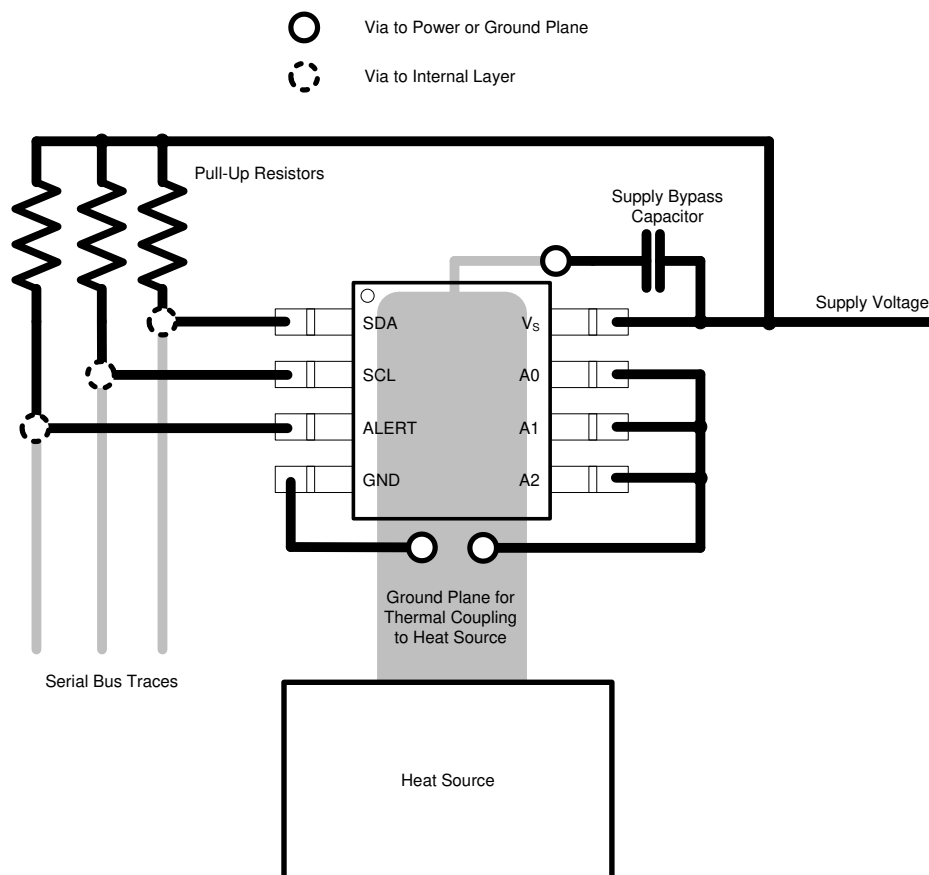
Figure 26. Layout Example
