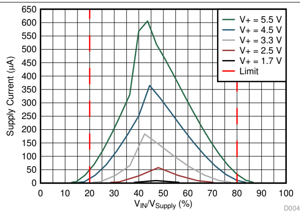
Figure 6. Supply Current vs Input Cell Voltage
