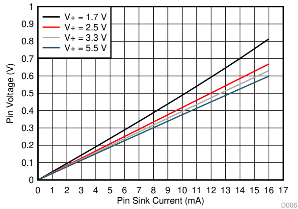
Figure 8. ALERT Pin Output Voltage vs Sink Current
