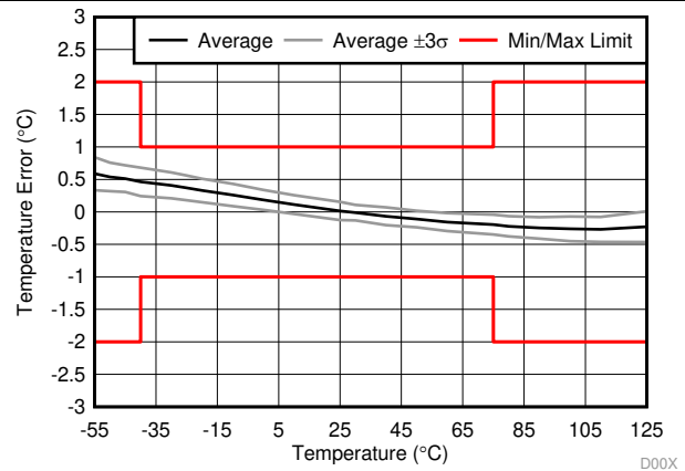
Figure 3. DSG Temperature Error vs Temperature
