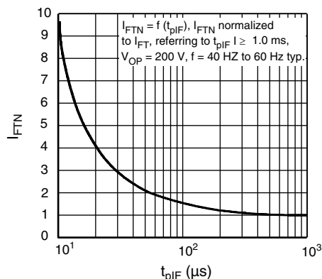
Fig. 10 - Pulse Trigger Current
