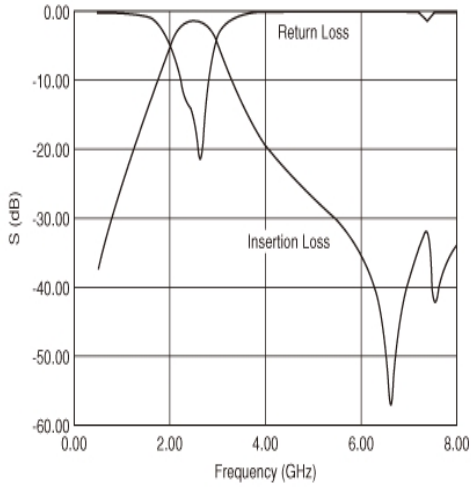
Frequency Characteristics
